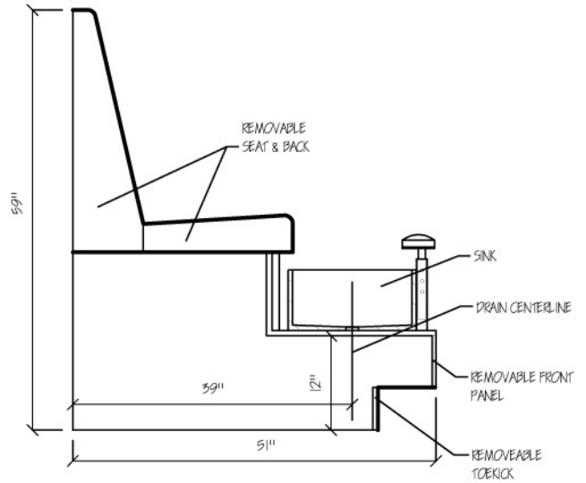
SIDE VIEW—PEDICURE BENCH
