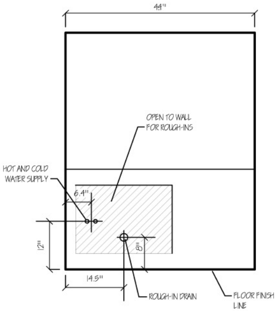
FRONT VIEW—SINGLE UNIT
