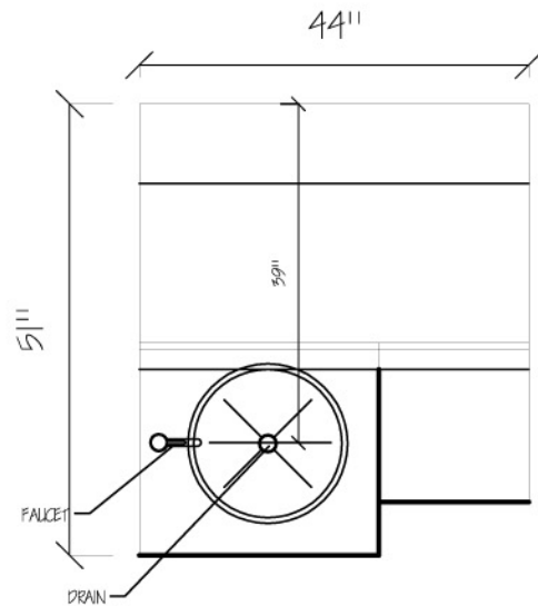
TOP VIEW—SINGLE UNIT
